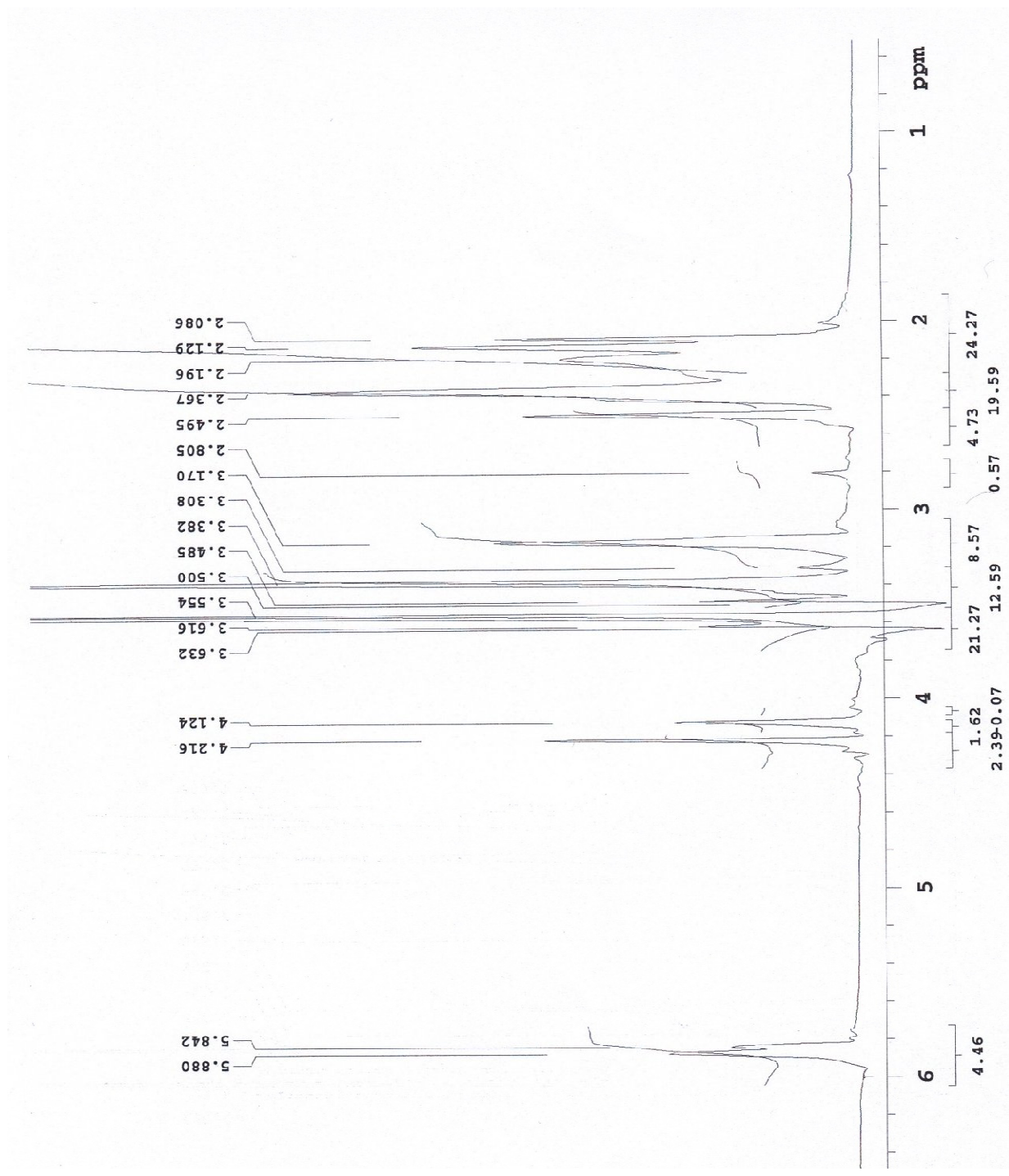
Figure 3.13: 1 H-NMR spectrum (AM-5)
